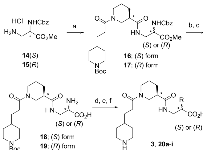
Scheme 2. Reagents and conditions: (a) 10 , EDC, HOBT, DMF, 93% for 16 , 96% for 17 ; (b) Pd–C/H 2 , MeOH; (c) aq LiOH, THF, 97% for 18 , 95% for 19 in two steps; (d) acylating reagent, MSA or aq NaOH (see Table 1); (e) HCl, EtOAc; (f) ODS column, then lyophilization (yields for 3 , 20a-i ; see Table 1).
