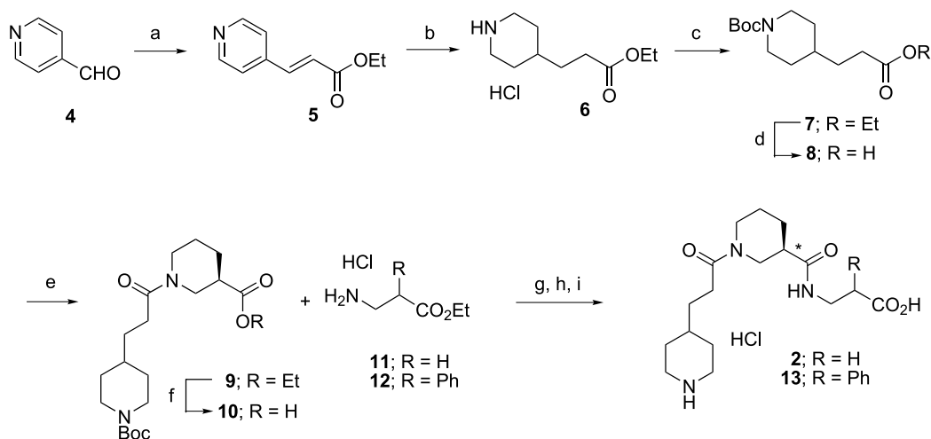
Scheme 1. Reagents and conditions: (a) (EtO) 2 POCH 2 CO 2 Et, NaH, THF, 78%; (b) PtO 2 , H 2 , HCl, EtOH, 88%; (c) (Boc) 2 O, Et 3 N, CH 2 Cl 2 , 81%; (d) aq NaOH, THF, EtOH, 91%; (e) ethyl ( R )-3-piperidinecarboxylate, EDC, HOBT, DMF, 86%; (f) aq LiOH, THF, EtOH, 90%; (g) EDC, HOBT, DMF; (h) aq LiOH; (i) HCl, EtOAc, 89% for 2 , 100% for 13 in three steps.
