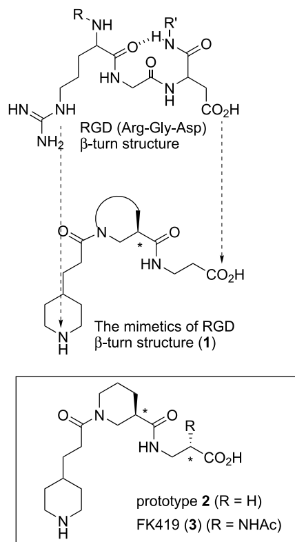
Figure 1. Design of prototype 2 from the structure of RGD \beta -turn peptide, and the structure of FK419 (3).
